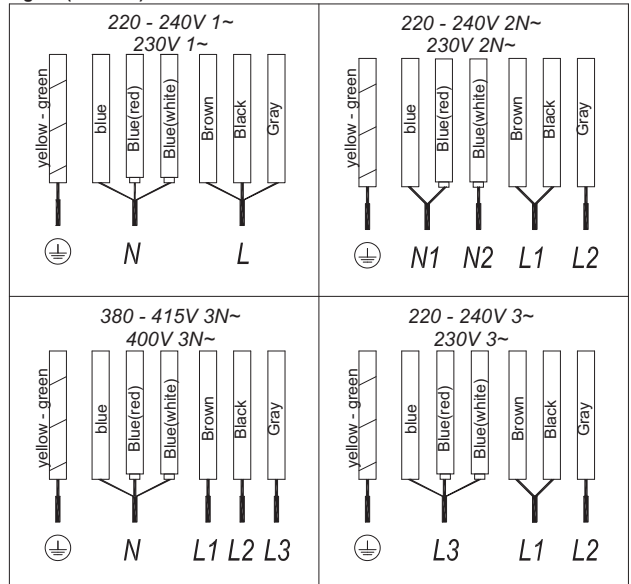
Fig. 2b (7 WIRES)
