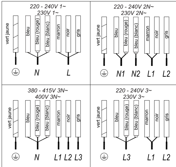
Fig.2b (7 FILS)
