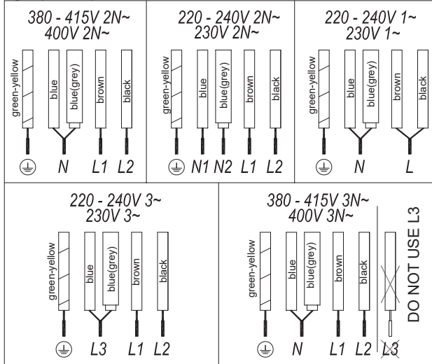
Fig.2a (5 WIRES)
