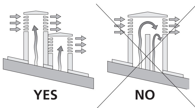
Fig. 4: chimney characteristics
